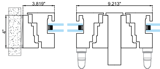
Horizontal Section
