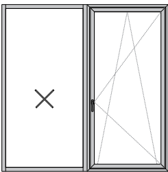
Single Sash + Fixed
